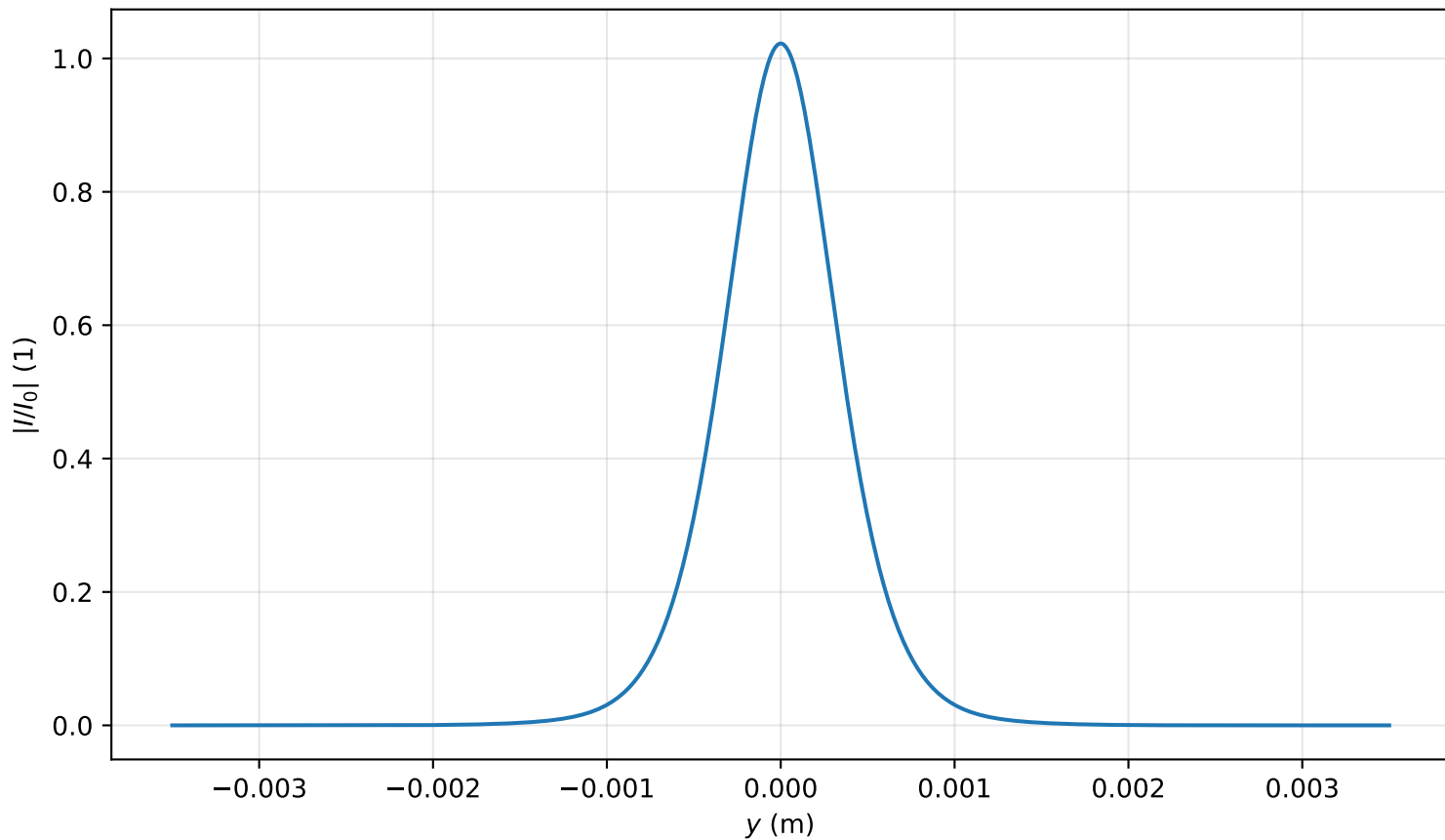
Intensity profile I(x=0, y, z=2.309)/I_0 , P_{in}=0.7P_{cr} , artificial time
